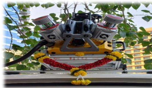
Trimble MX-90
